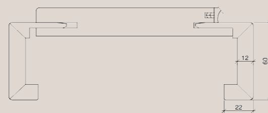
Detail Zarge P60/22
