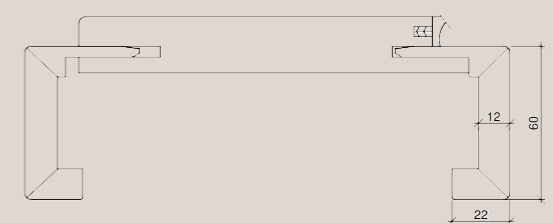
Detail Zarge P60/22
